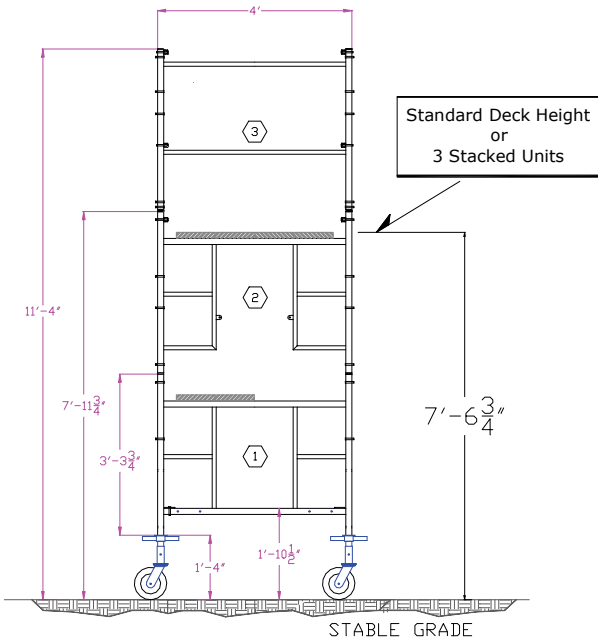
Model 3948M.A2 Scaffold (Standard Unit Overall Height)
