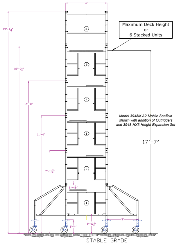
Model 3948M.A2 Mobile Scaffold Maximum Freestanding Height
