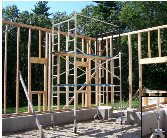
EASY ASSEMBLY – Starting with End-Frame Units, Cross Braces, Diagonal Brace, Hand Rails and Frame Leveler Jacks with Swivel/Locking Casters.
